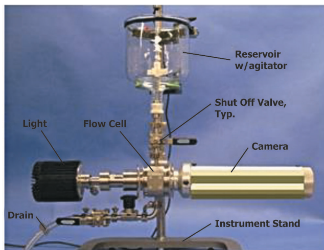
FIG. 1 Example Arrangement of a Flow Cell
